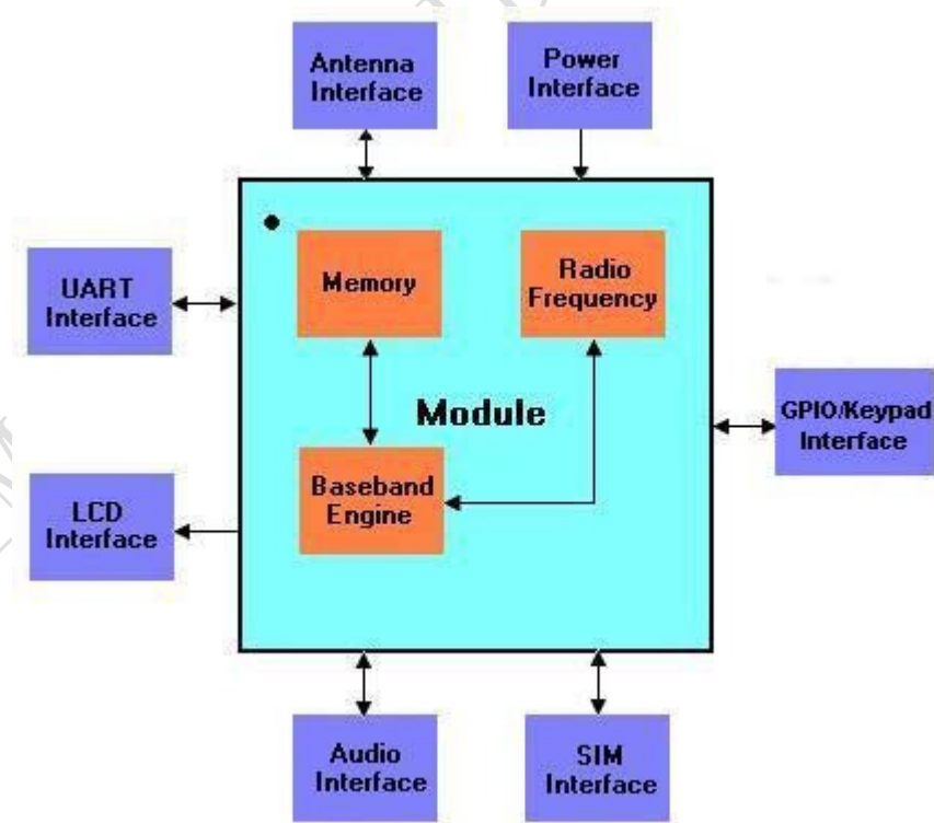
Figure 1: SIM900 functional diagram
