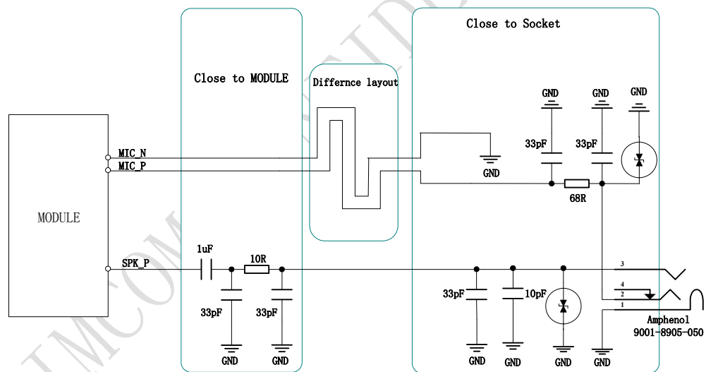
Figure 26: Earphone interface configuration
