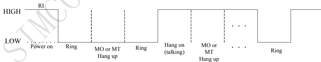
Figure 33: SIM900 Services as Receiver
