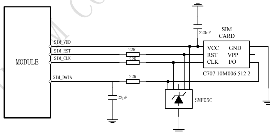
Figure 28: Reference circuit of the 6 pins SIM card
