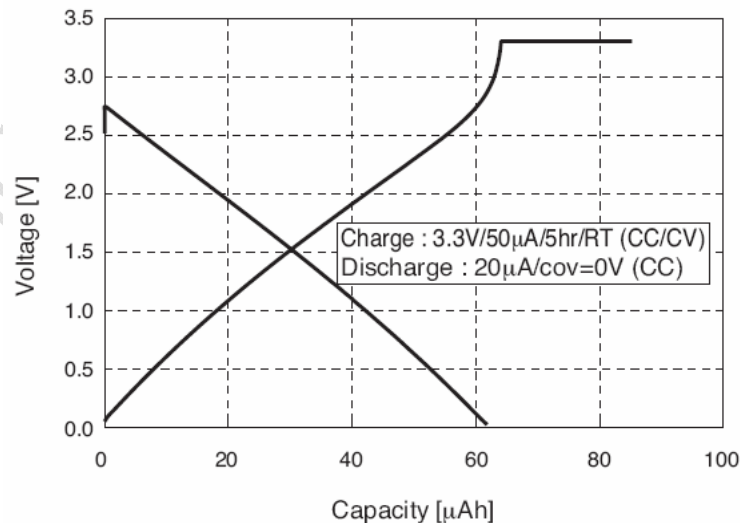
Charge-Discharge Characteristics
