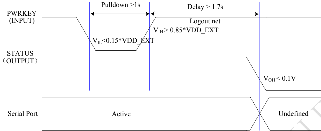
Figure 12: Timing of turn off system using PWRKEY
