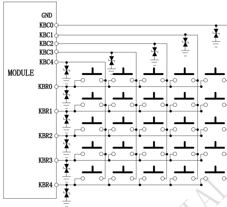
Figure 31: Reference circuit of the keypad interface
