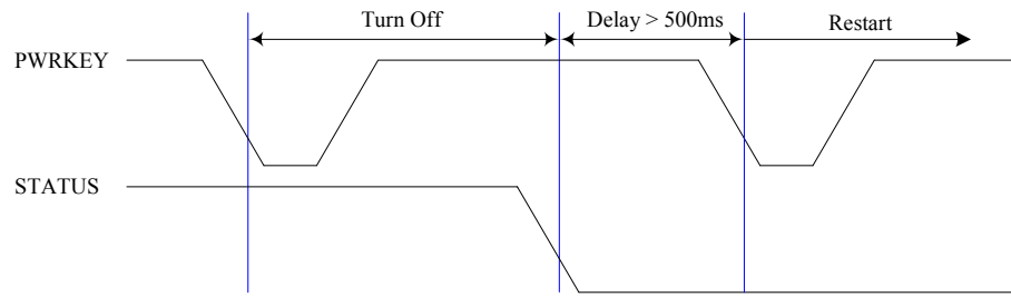
Figure 14: Timing of restart system
