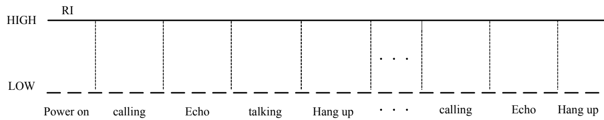
Figure 34: SIM900 Services as caller
