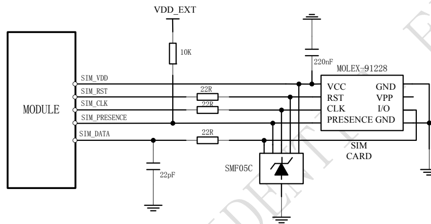
Figure 27: Reference circuit of the 8 pins SIM card
