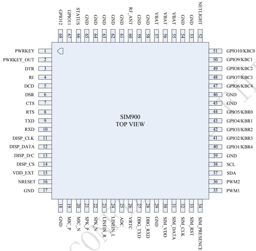
Figure 41: SIM900 pin out diagram (Top View)
