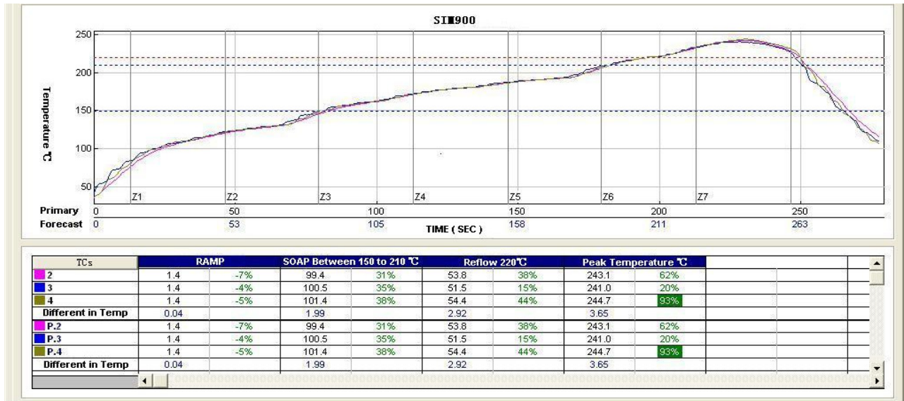
Figure 42: The ramp-soak-spike reflow profile of SIM900
