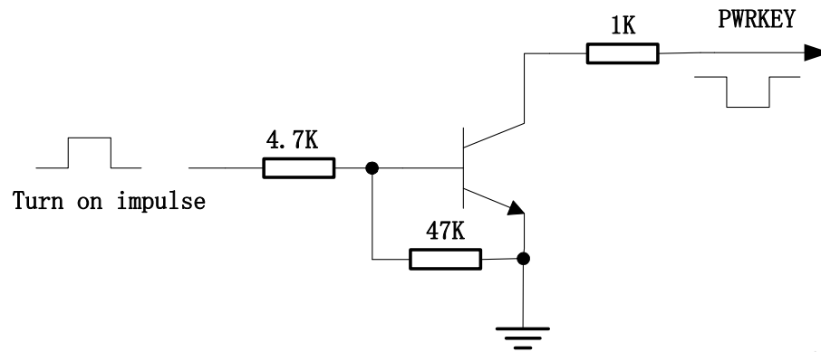
Figure 6: Turn on SIM900 using driving circuit
