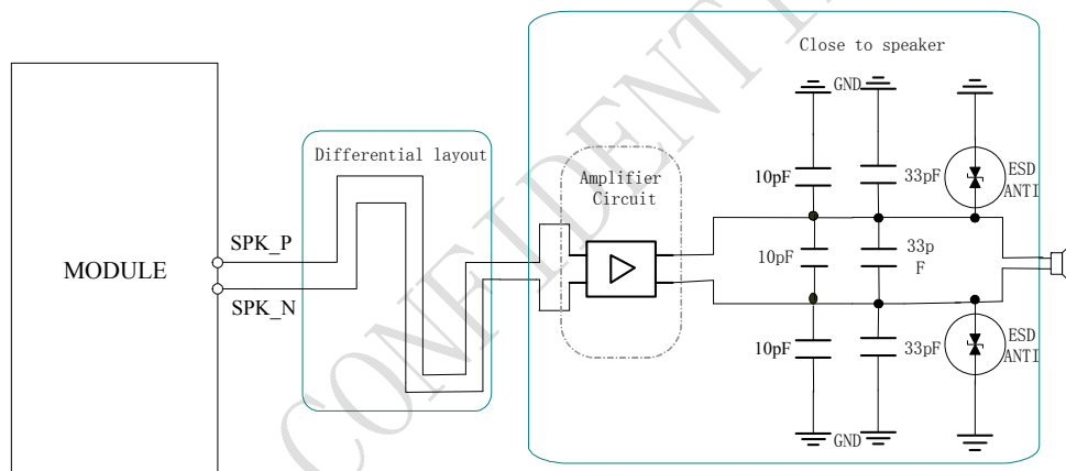
Figure 24: Speaker interface with amplifier configuration
