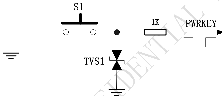
Figure 7: Turn on SIM900 using button
