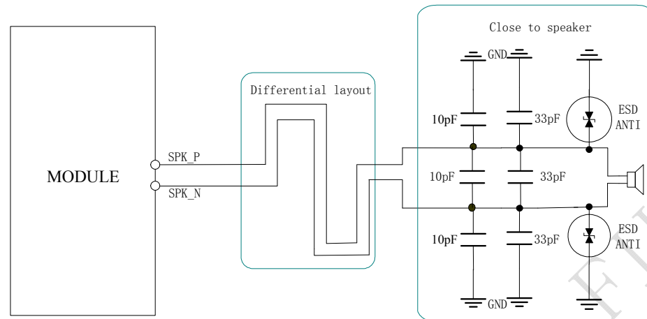
Figure 23: Speaker interface configuration
