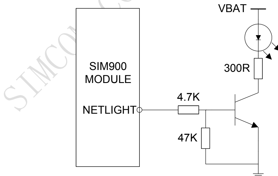
Figure 35: Reference circuit of NETLIGHT
