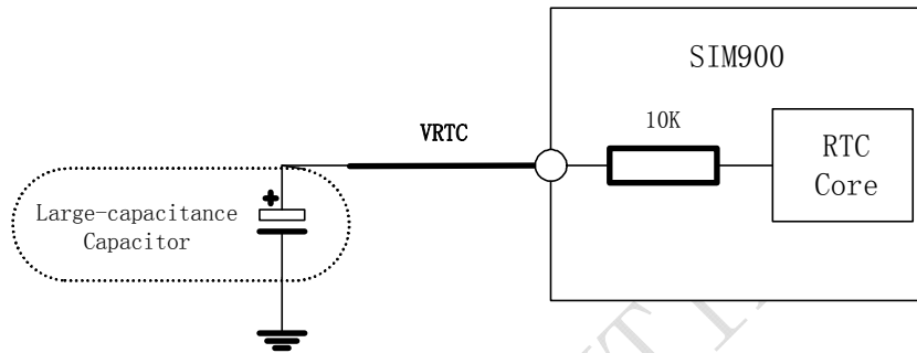
Figure 18: RTC supply from capacitor
