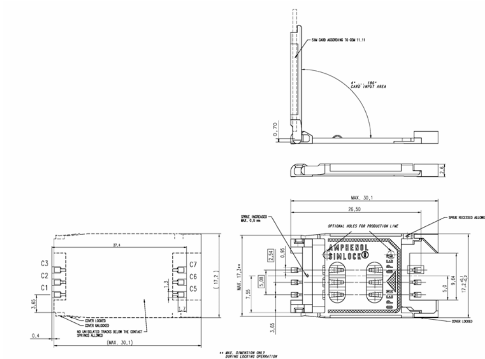
Figure 29: Amphenol C707 10M006 512 2 SIM card holder
