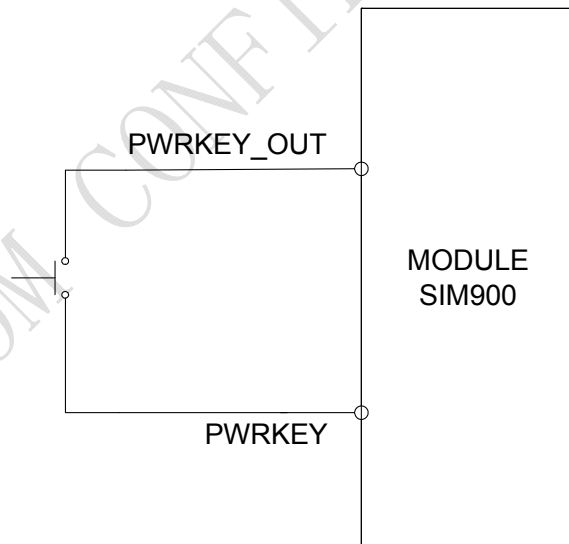
Figure 10: Turn on SIM900 using button
