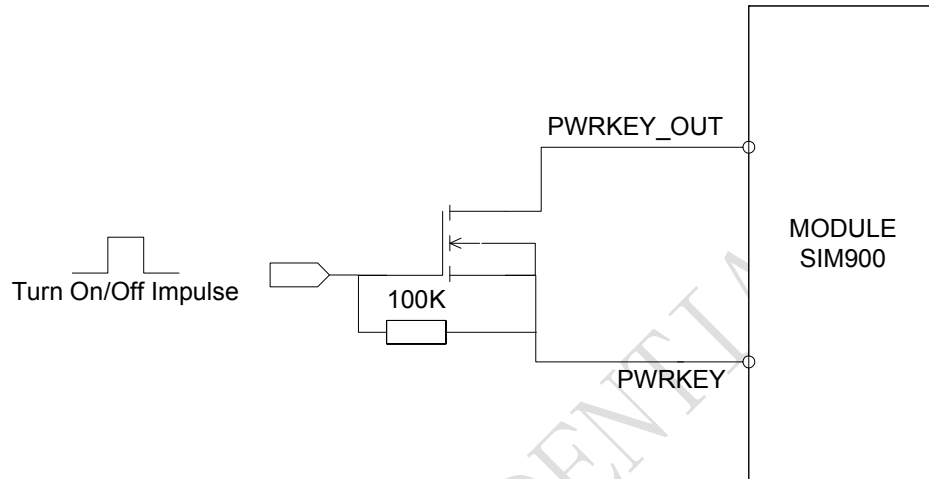
Figure 9: Turn on SIM900 using driving circuit
