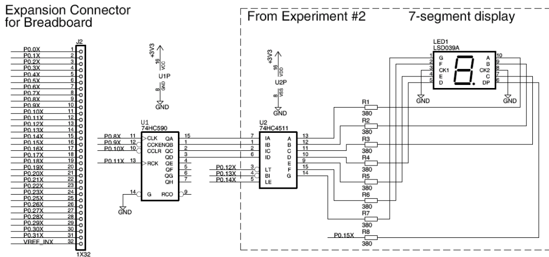
Figure 17 – Experiment #3: Counter
