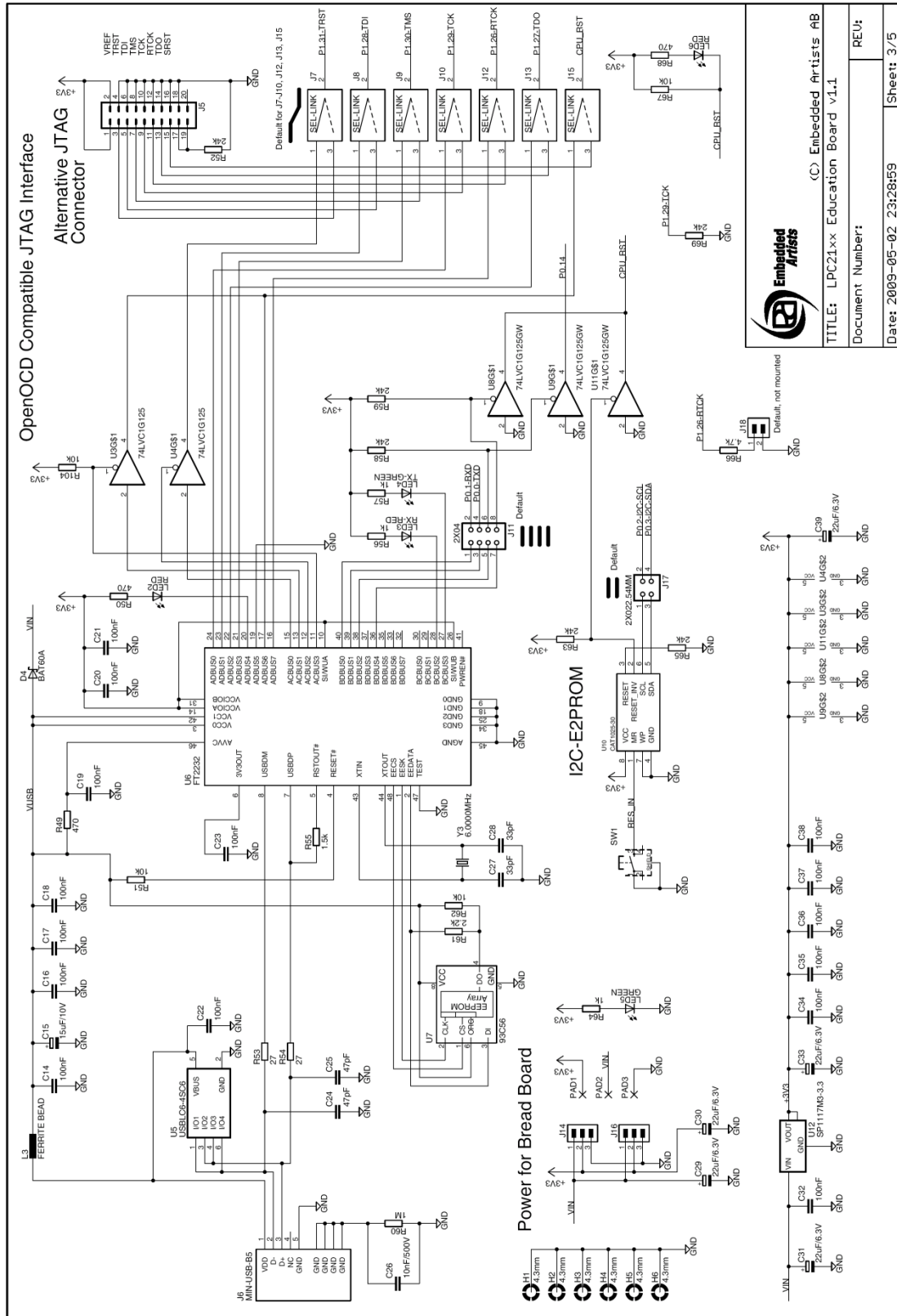
Figure 4 - LPC2138 Education Board Schematic, Page 3
