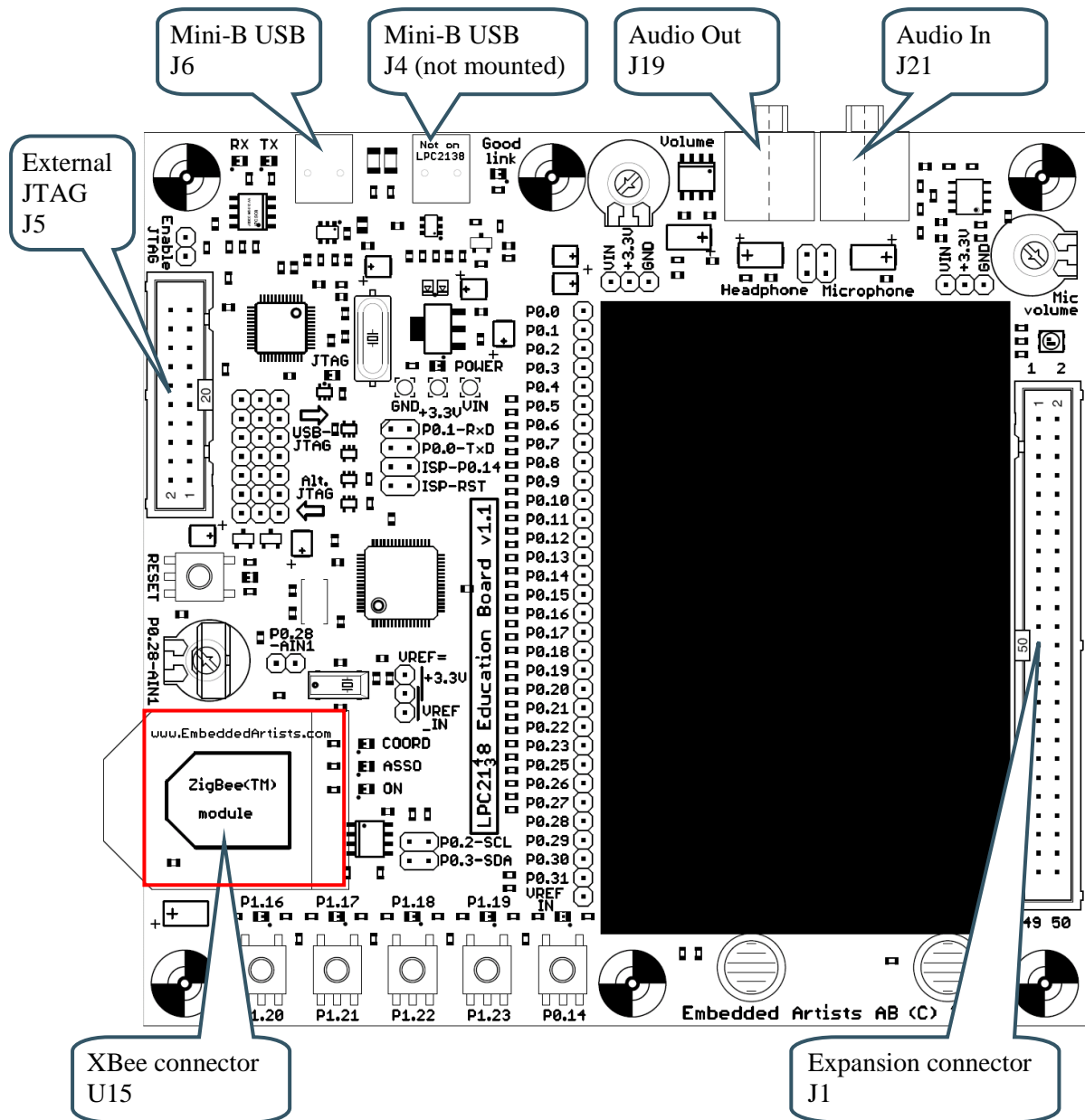
Figure 8 - LPC2138 Education Board External Connectors
