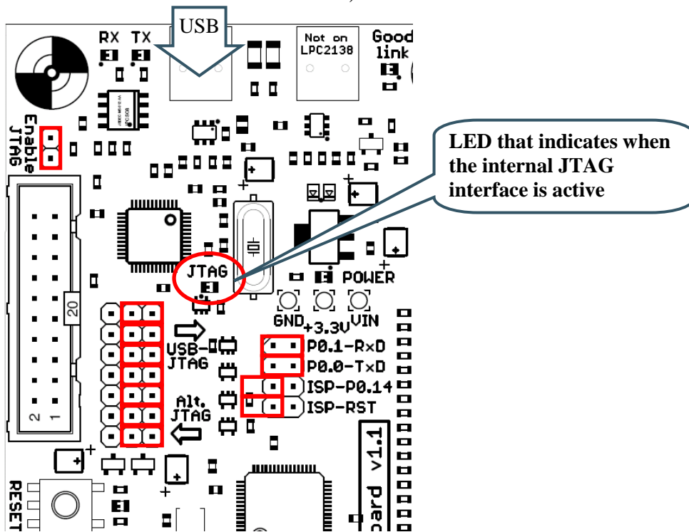
Figure 22 – JTAG and ISP Jumpers, enable internal JTAG
