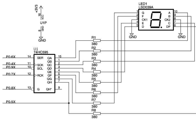
Figure 18 – Experiment #4: Shift Register
