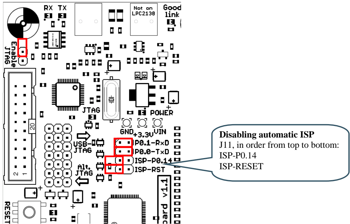
Figure 27 – ISP Jumpers, disable automatic ISP
