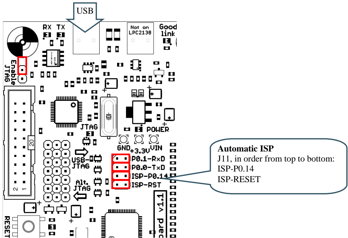
Figure 26 – ISP Jumpers, enable automatic ISP
