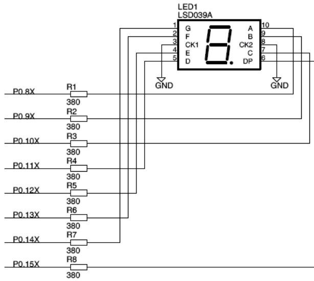
Figure 13 – Experiment #1: 7-segment LED Display
