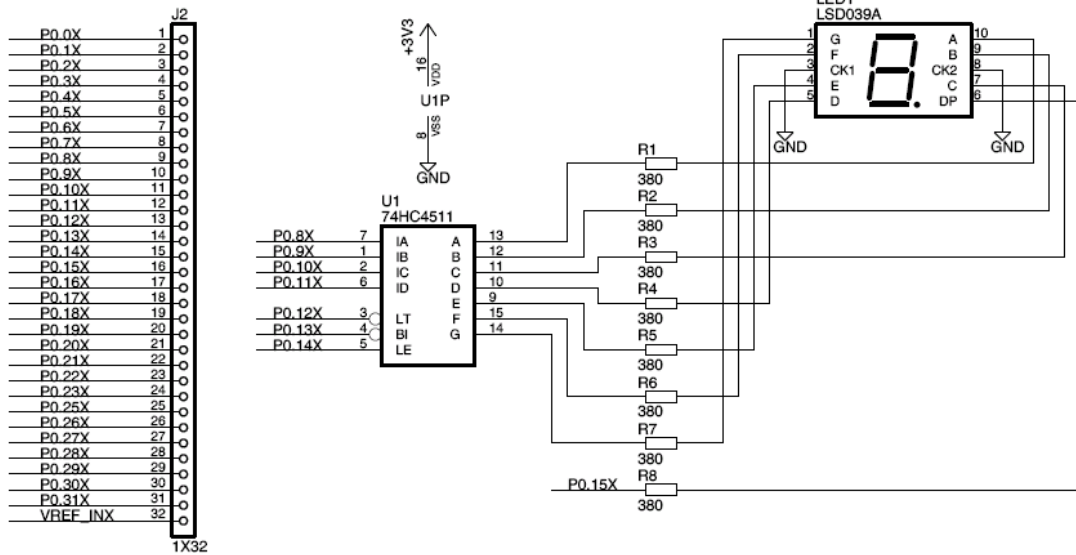
Figure 15 – Experiment #2: 7-segment Decoder
